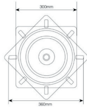
材质厚度:2.5/3.0mm 尺寸/Size:300x300mm转盘
