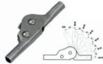
C-216-1正五档90° 日本扣 Single gear wheel hinge
