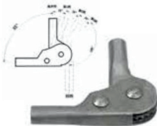
C-216-4反三档日本扣 Flat gear wheel hinge
