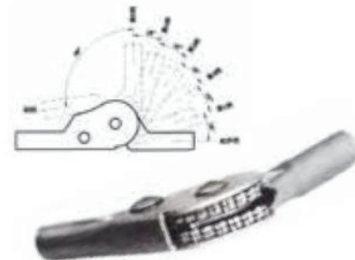
C-216-7双齿日本扣 Double gear wheel hinge
