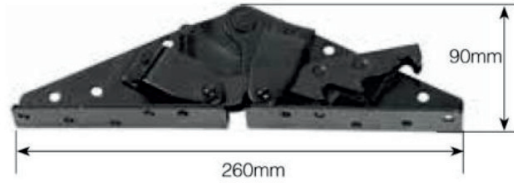
C-12-2中型沙发铰 Small Double-use hinge
