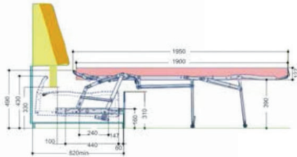
C-73B二折沙发床/2 Folds bed
