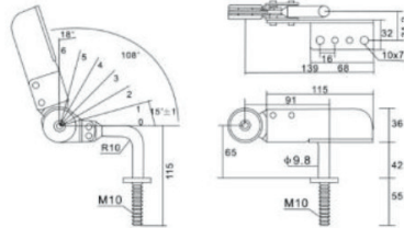
C-308A单边长耳
